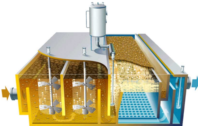
Figure 5 | Typical AquaDAF ® tank configuration (courtesy of IDI).
