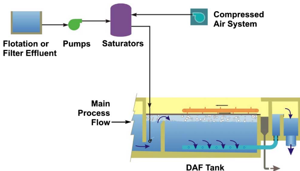
Figure 2 | Typical DAF recycle system.
