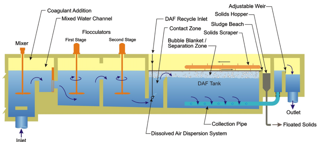
Figure 1 | Typical DAF system schematic.
