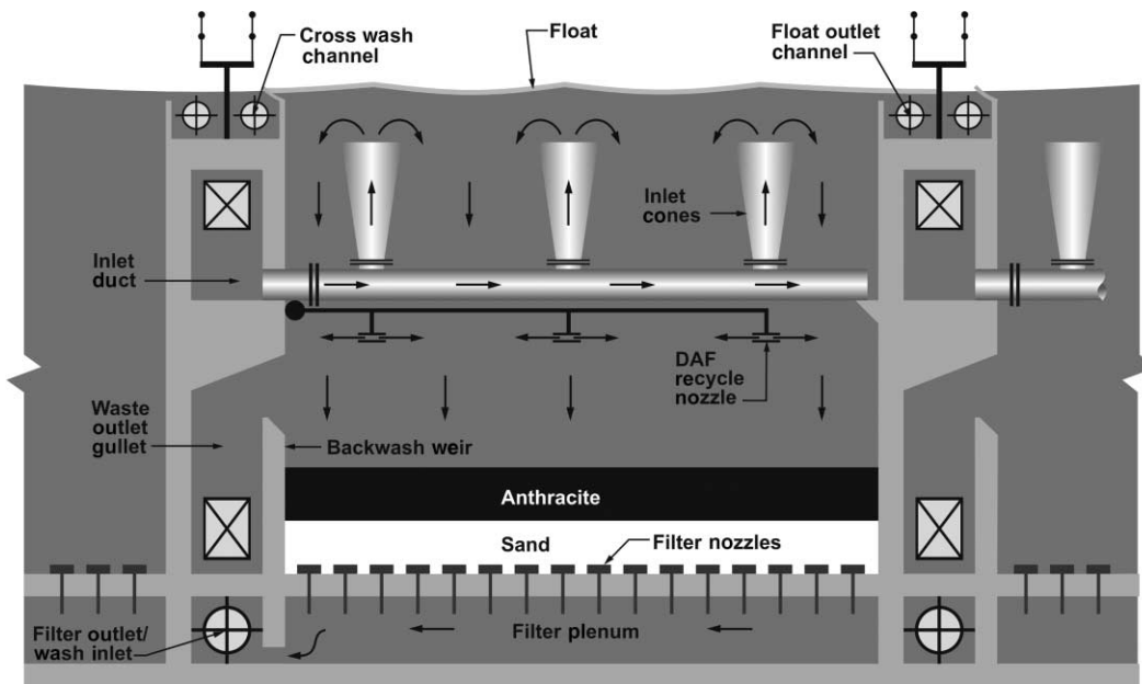
CoCo DAF™ cross section schematic
